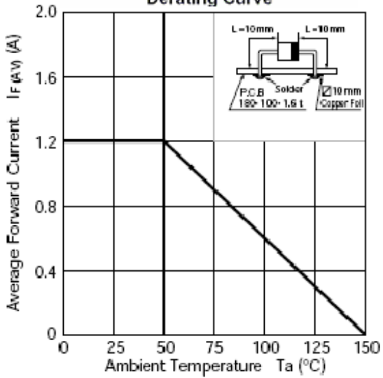
Fig. 1 – Maximum Forward Current Derating Curve
